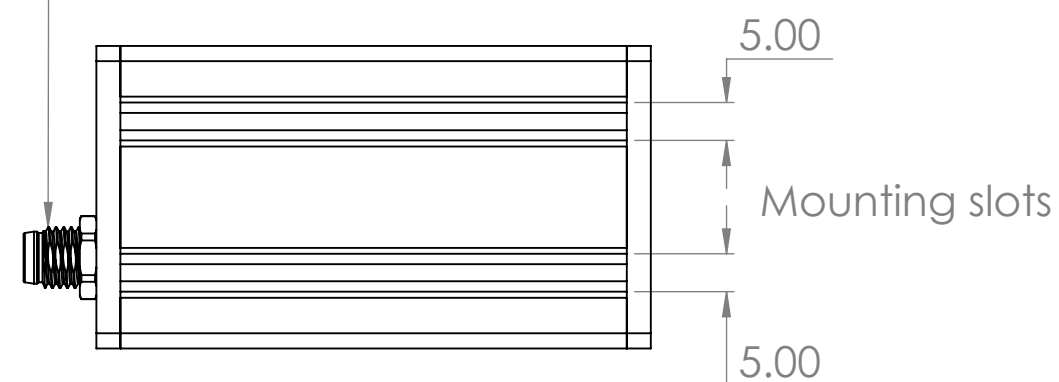
M8 Connector - Code A
